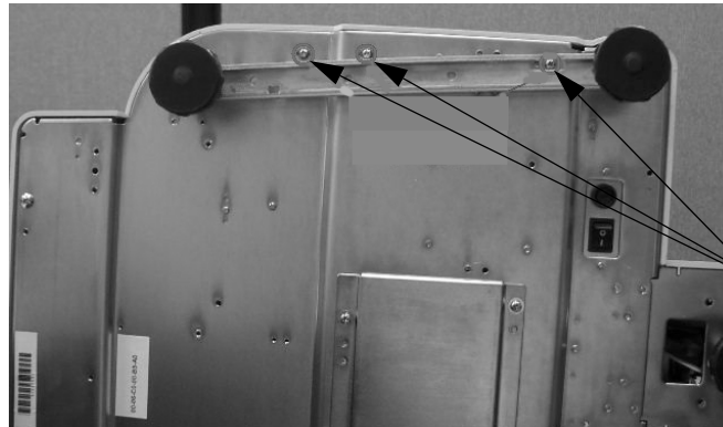
Figure 2-4. DC200 Screw Location
