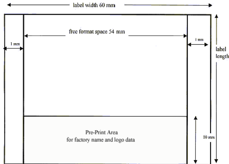
Figure 7-37. Free Format Label Print Areas Available
