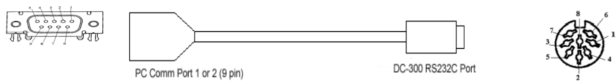
Figure 12-2. Connection from Scale to PC
