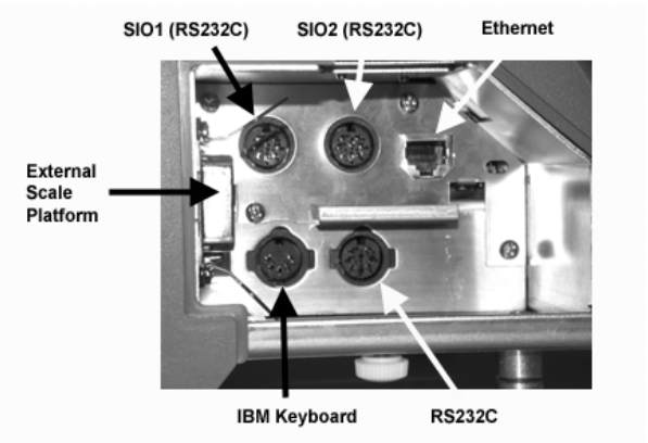
Figure 12-5. Keyboard Port Location
