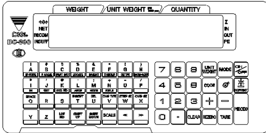
Figure 1-2. DC-200/300 Display
