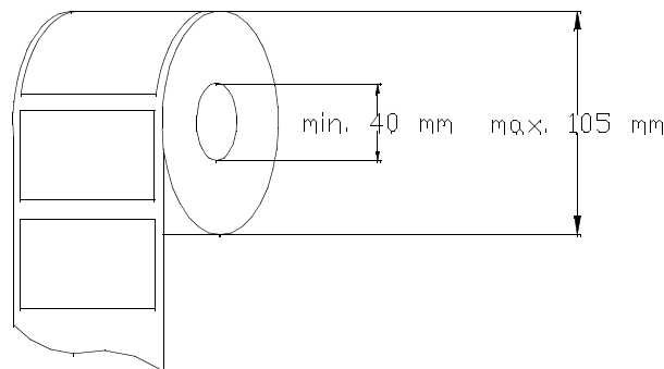
Figure 7-1. Label Roll Dimensions
