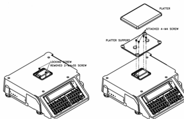
Figure 2-1. Unlocking the Scale and Installing the Platter Support
