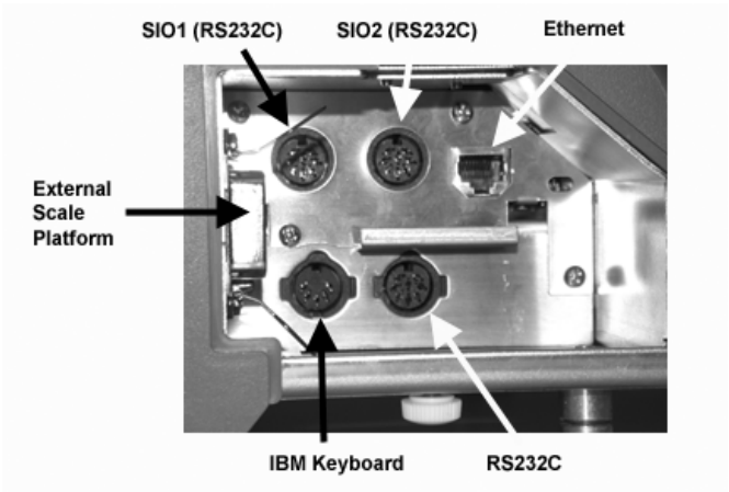
Figure 12-1. DC-200/300 Interface Ports
